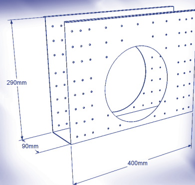
TJD290 (for 290 X 90mm joist)
