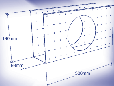
TJD190 (for 190 x 90mm joist)
