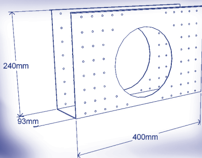
TJD240 (for 240 x 90mm joist)
